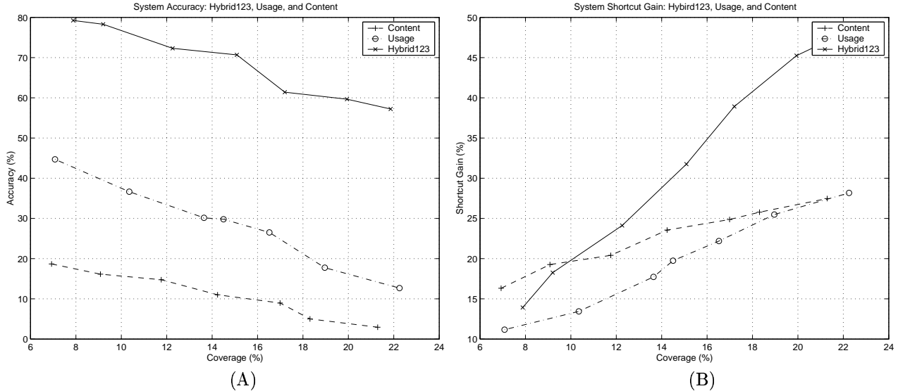
Figure 3. Hybrid123, Usage, and Content. (A): Recommendation Accuracy (B): Shortcut Gain
