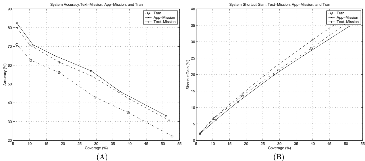
Figure 5. Text-Mission , App-Mission , and Tran . (A): Recommendation Accuracy (B): Shortcut Gain
