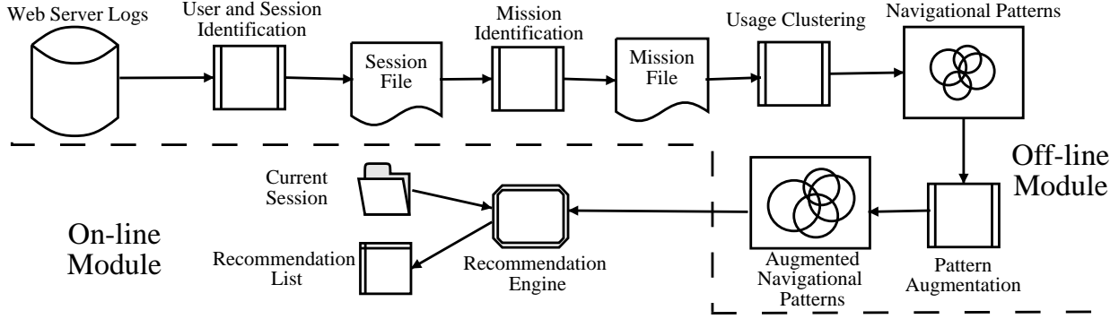
Figure 1. System Architecture
