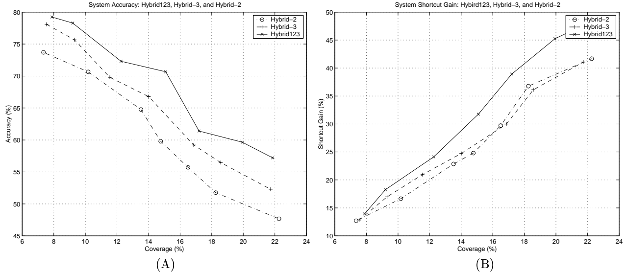
Figure 4. Hybrid123 , Hybrid-3 , and Hybrid-2 . (A): Recommendation Accuracy (B): Shortcut Gain
