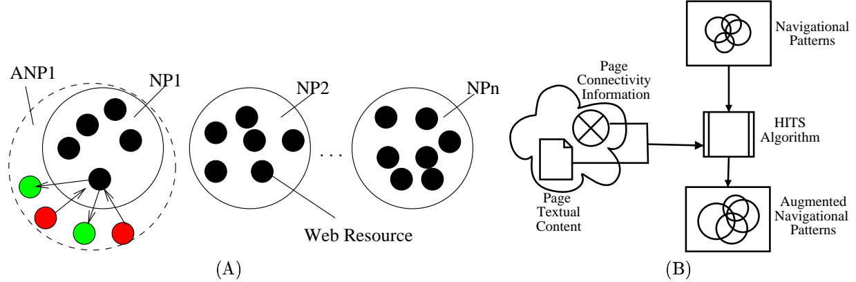
Figure 2. (A) Navigational Patterns(NPs) and Augmented Navigational Patterns(ANPs) (B) Augment Process
